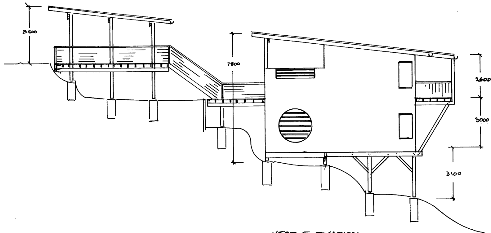
WEST ELEVATION
