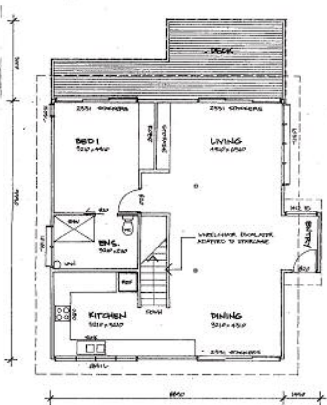
2 UPPER FLOOR
