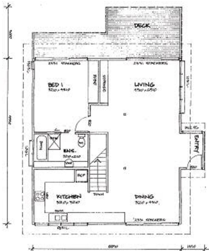
2 UPPER FLOOR
